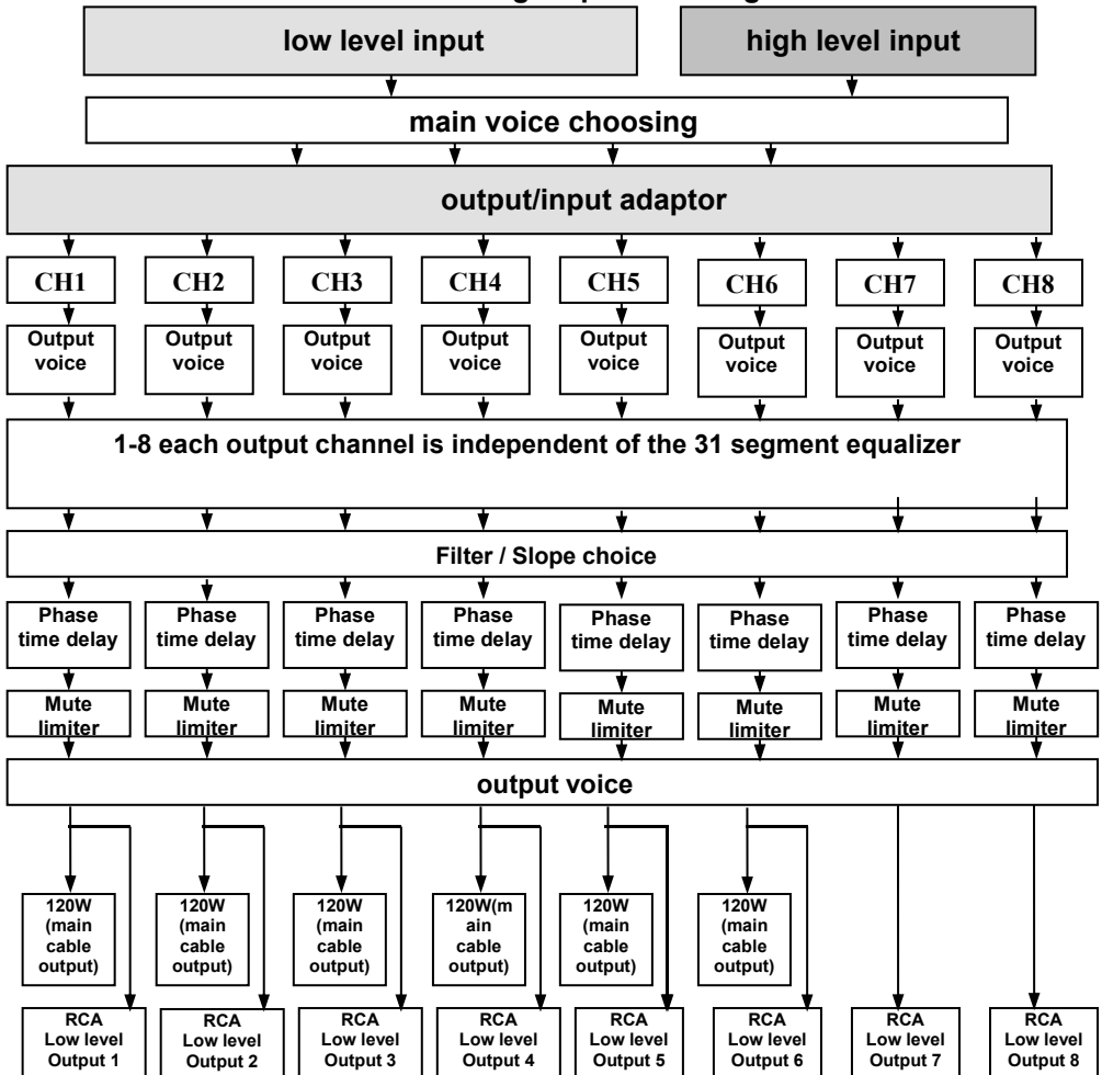
Main audio signal process diagram
